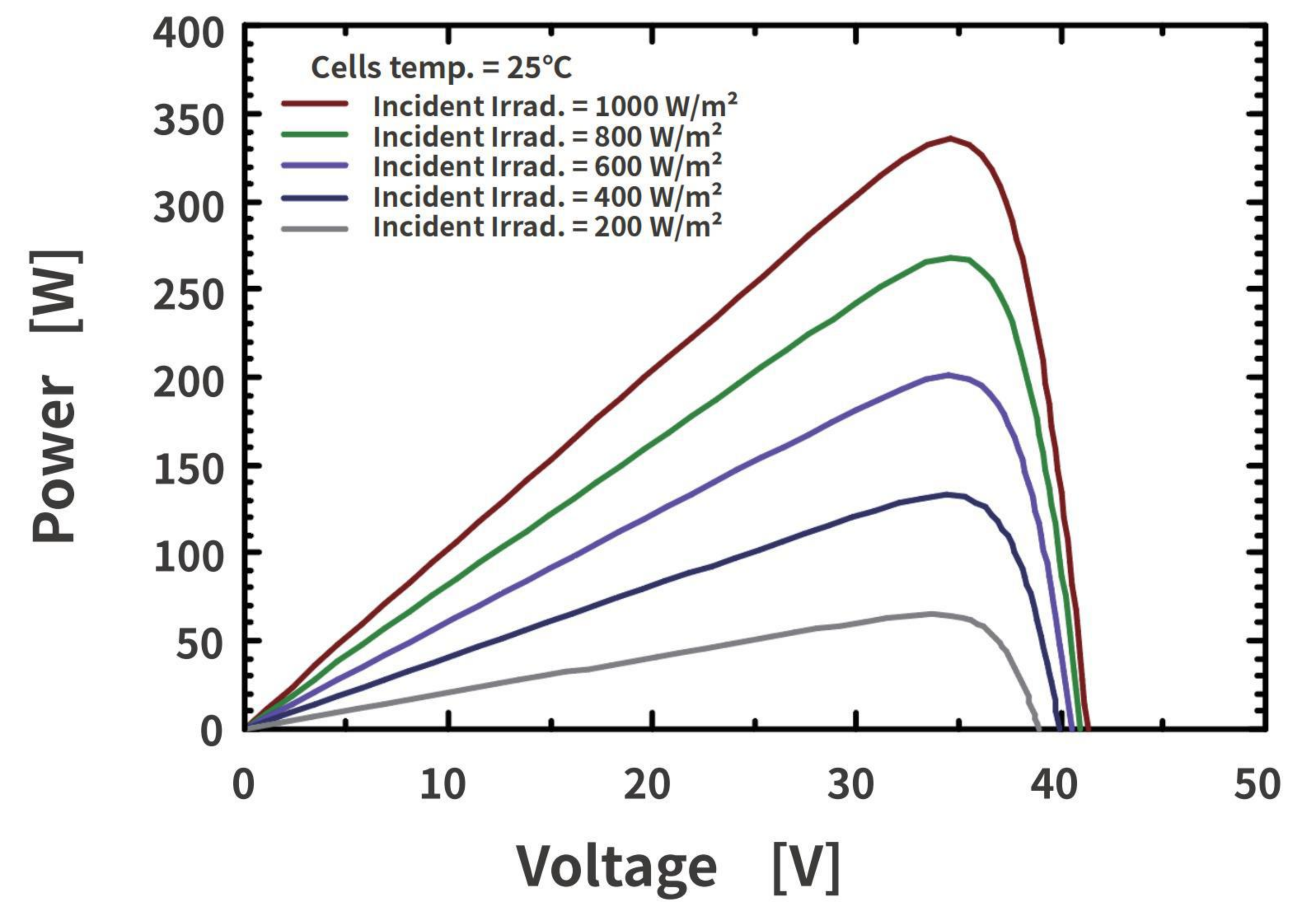
P-V Curves of PV Module
